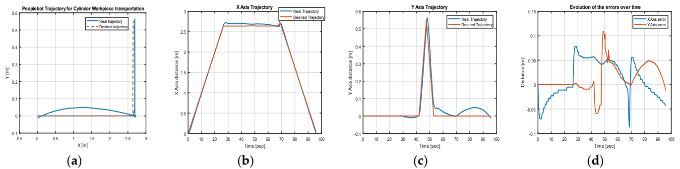
Figure 24. CAS's DT-TTSMC for cylinder recovery: (a) desired and real trajectory; (b) along the X axis; (c) along Y axis; (d) errors.
