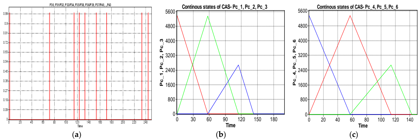
Figure 15. (a) The monitoring signals for the successive actions of the WP2 repair. (b) The continuous places evolution of the CAS (PeopleBot WMR), places: P_{c\_1}, P_{c\_2}, P_{c\_3} for replacing cylinder 1. (c) The continuous places evolution of the CAS, places: P_{c\_4}, P_{c\_5}, P_{c\_6} for replacing cylinder 2.
