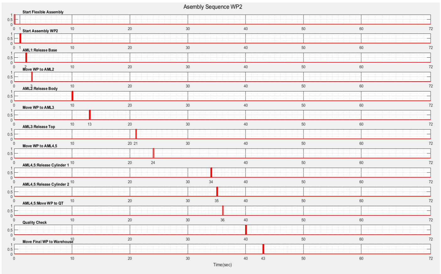
Figure 20. Real-time monitoring signals corresponding to assembly operations of WP2.
