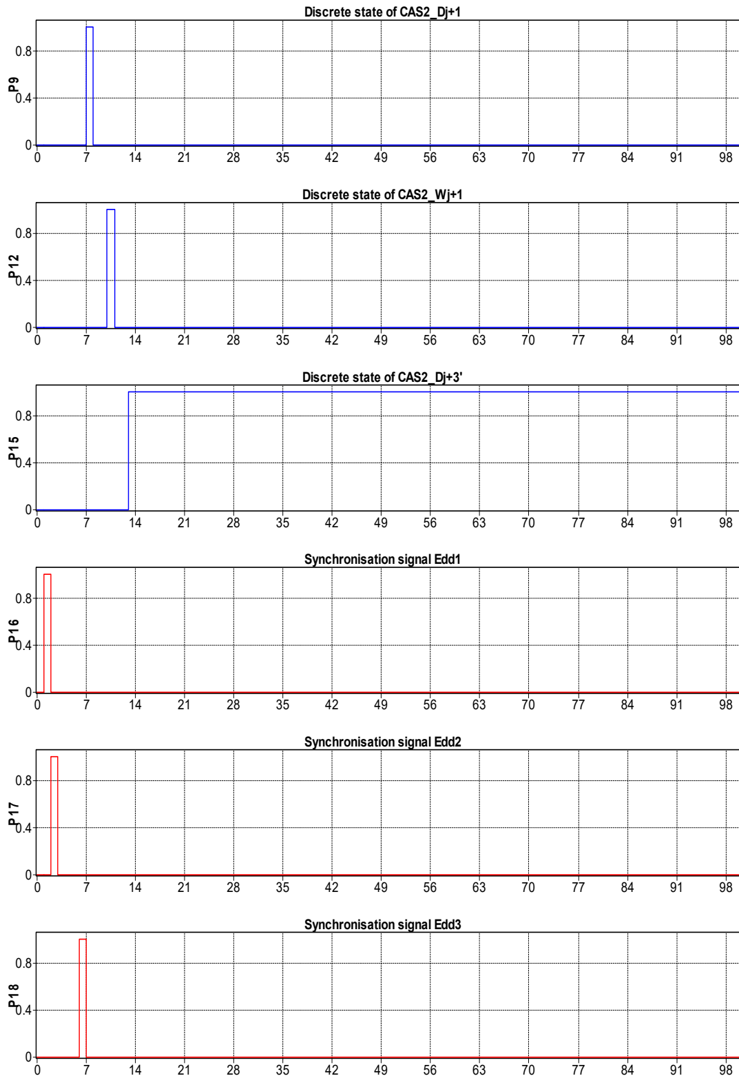
Figure 14. Discrete states of disassembled work piece, CAS1 and CAS2 in relation with synchronization signals for collaborative actions.
