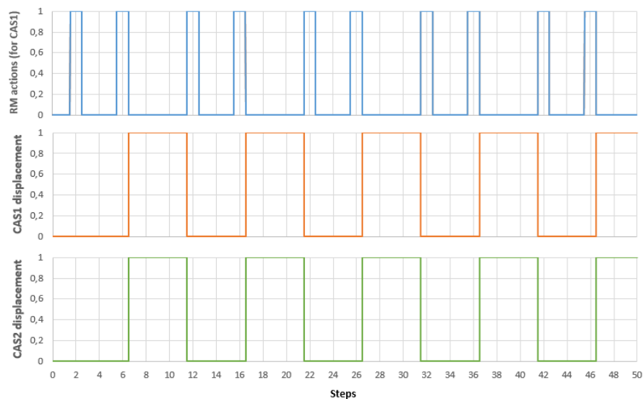
Figure 21. Control of CAS1 and CAS2 synchronized movement, correlated with manipulation tasks, in a complete disassembly cycle.
