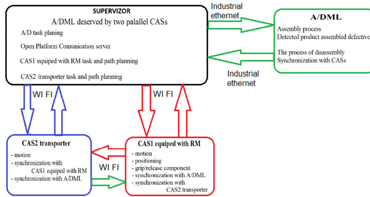
Figure 19. Data workflow in real-time control mode.
